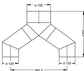
Kit de raccordement (Dimensions)
